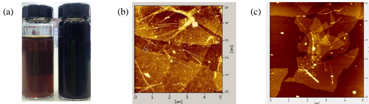
FIGURE 2. (a) physical state of GO and rGO; and AFM images (b) GO; (c) rGO.
