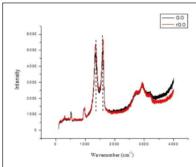
FIGURE 4. Raman spectra for GO and rGO.
